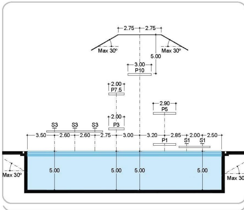
Diving Marking Lanes - Distance A: The centre of the first line shall be directly under the plummet of the 3 metre Springboard.
